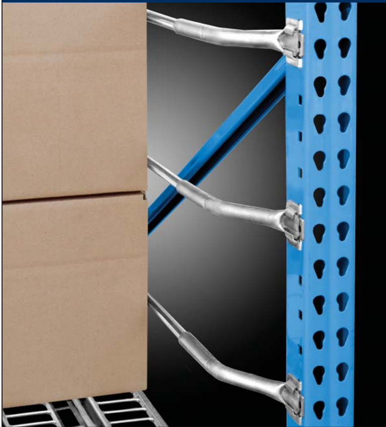
Provides 3" clearance between rack and stored material
